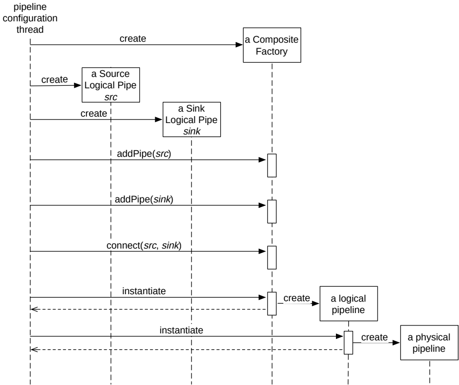
Fig. 10. A UML Sequence diagram showing how a physical pipeline is created
