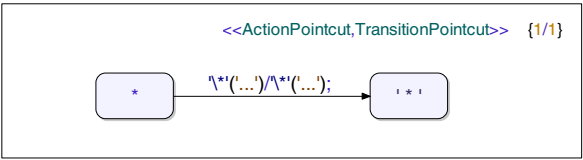
Fig. 6. A WEAVR pointcut descriptor
