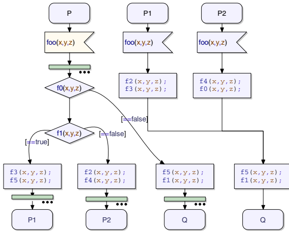
Fig. 14. Isolation of the selection matching pct(P \rightarrow^{foo} (P1 \text{ OR } P2 \text{ OR } Q)) . The behavior that is common to paths that do not match the pointcut has been replicated to apply the after advice correctly.
