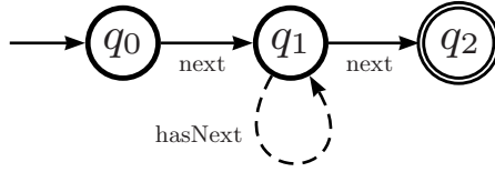
Fig. 3. Finite automaton for tracematch pattern HasNext
