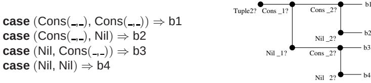
Fig. 6. Optimizing nested patterns
