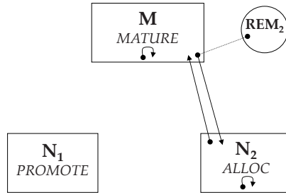
Fig. 3. Edges added outside of a nursery collection
