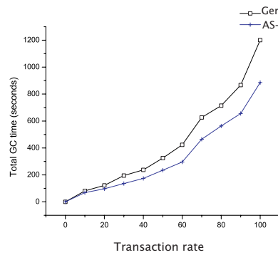
Fig. 8. Comparing overall collection times
