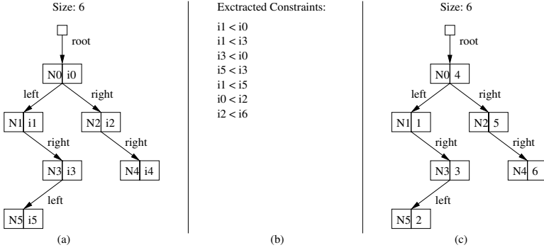
Fig. 5. (a) BinarySearchTree object repaired by Juzi++; primitive fields have symbolic values. (b) Difference constraints on primitive fields computed by Juzi++. (c) Solution to the constraints generated by Dicos used to assign values to the primitive fields.
