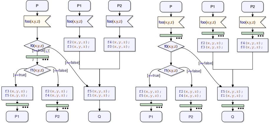
Fig. 13. (a) Selection for pct(P \xrightarrow{foo} (P1 \text{ OR } P2)) . (b) Selections for pct((P \text{ OR } P1 \text{ OR } P2) \xrightarrow{foo} *) .
