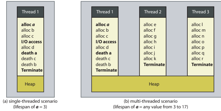
Fig. 15. What is the lifespan of object a ?
