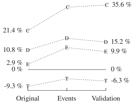
Fig. 19. Reduction Compared to Java
