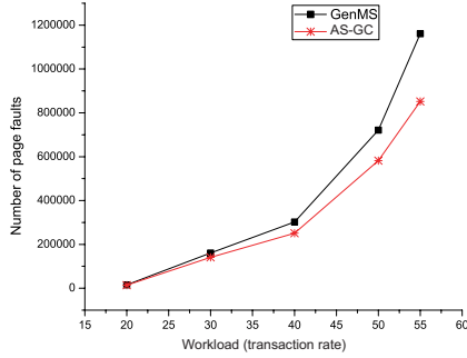
Fig. 13. Comparing paging behavior under heavy workloads
