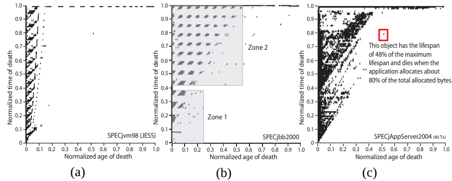
Fig. 1. Each dot in these graphs represents an object. The x-axis represents the normalized age of death, and the y-axis represents the normalized time of death. Thus, the position of each dot provides us with the age of that particular object and the time that it dies. For example, the squared object in the SPECjAppServer2004 graph (c) has a lifespan of 48% of the maximum lifespan and dies when the application allocates about 80% of the total allocated bytes.
