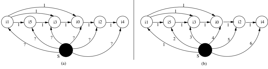
Fig. 6. (a) Data constraint graph based on the constraints from Figure 5 (b); the edges labeled with weight 1 arise from the difference constraints; S is the new reference node and edges labeled with ‘?’ indicate the new edges. (b) Solution for the difference constraints; each ‘?’ has been replaced with the value of the longest distance from S.
