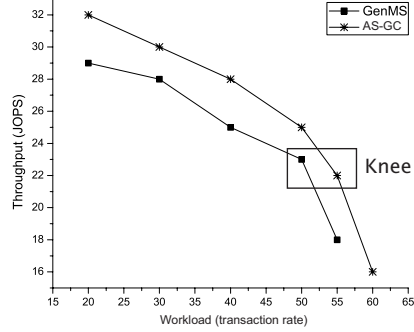
Fig. 14. Comparing throughput degradation locations
