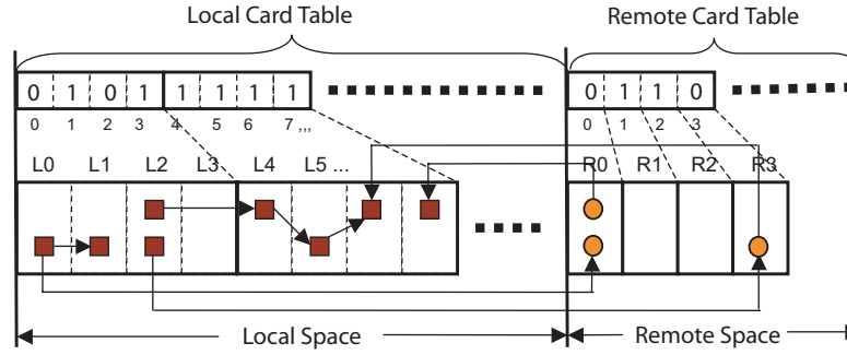
Fig. 6. Each round object represents a remote object, and each square object represents a local object. The nurseries are divided into 128-byte blocks; each block is represented by one byte card allocated in a separated card table area. Initially, each byte is set to the value of 1. When an inter-nursery reference is made (write-barrier is used to detect such a reference), the card representing the memory block that contains the inter-nursery reference becomes dirtied and is assigned the value of 0. In the example shown here, there are four inter-nursery references originated from memory blocks L0, L2, R0 and R3; thus, those cards have the value of 0.
