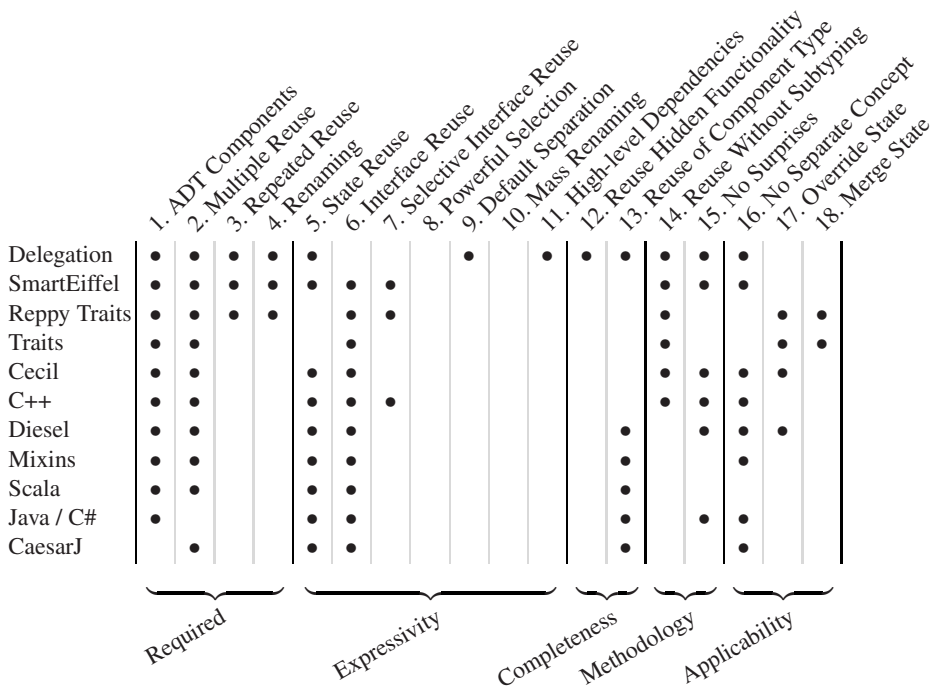
Fig. 3. Feature matrix for different code reuse mechanisms
